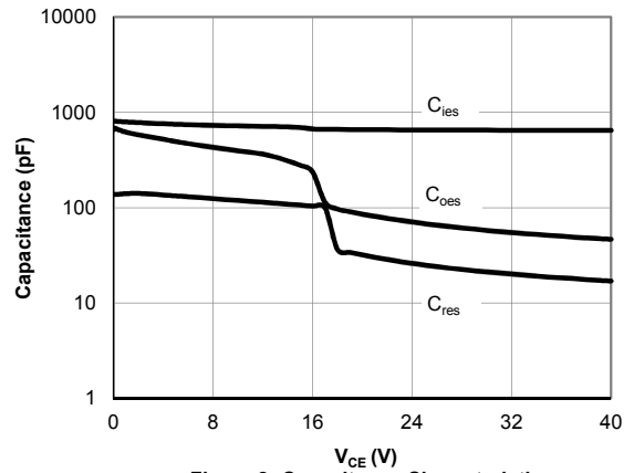
Figure 8: Capacitance Characteristic
