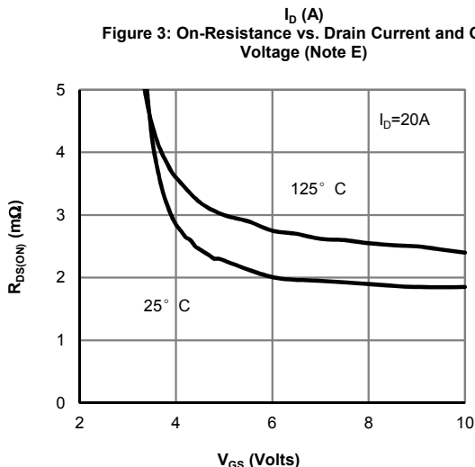
Figure 5: On-Resistance vs. Gate-Source Voltage (Note E)
