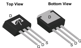
TO-262
