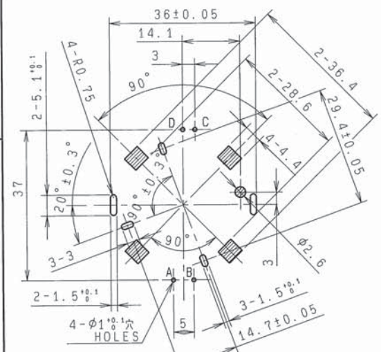
端子先端形状 TERMINAL DETAIL
