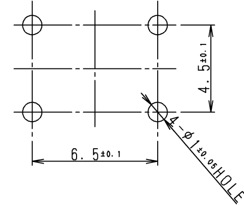
プリント基板取付穴寸法図 (スイッチ取付面より見る) Printed Circuit Board Mounting Hole Dimensions (When viewed from switch mounting face)
