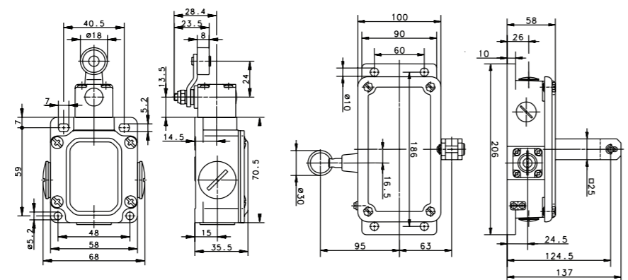
SN2 Limit Switch without Cable
