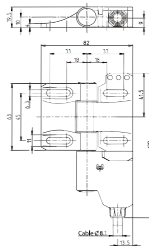
SHS3...KA...
