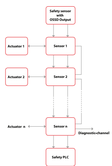
Series application
