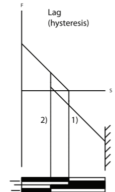
Fig. 3 shows the contact force during the switching cycle of a snap-action contact.
