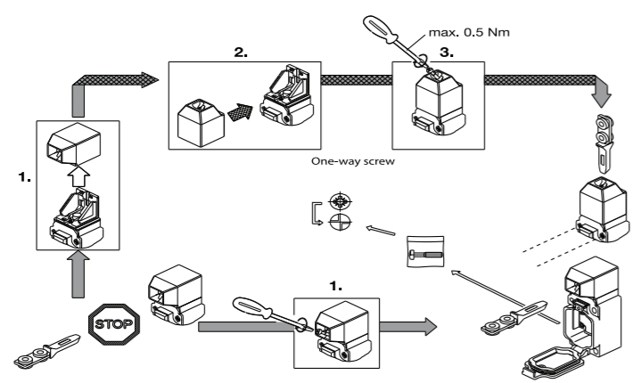
Repositioning the actuator head either in horizontal or vertical direction results in 8 approach actuator directions.
