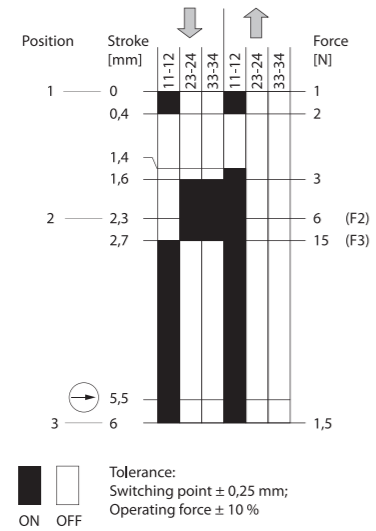
Switching diagram
