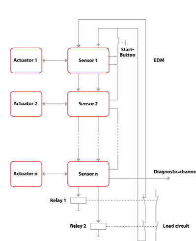
Series application
