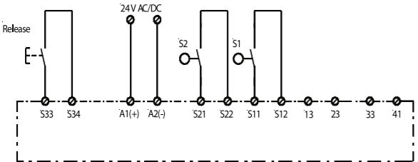
Schematic representation of safety relay system
