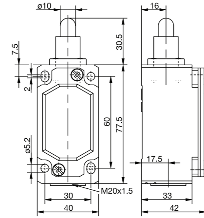
IW (Form B)
