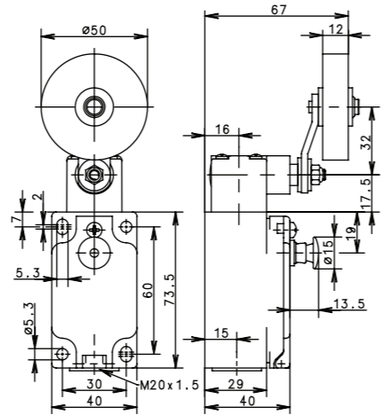
AHS-GU RAST R0050 - LATCHING
