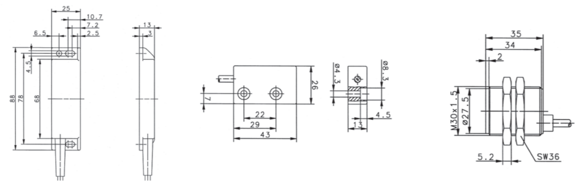
Drawing dimensions in mm
