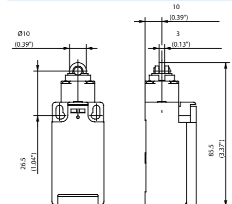
RIWK (Form C)
