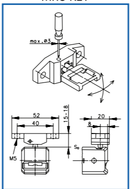
MRU KEY
