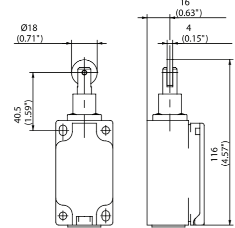
RIW (Form C)
