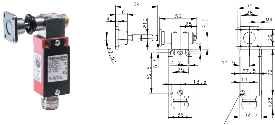
Blind hole for fitted pin Ø4 ; 5.5 deep
