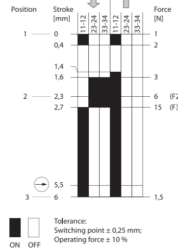
Switching diagram
