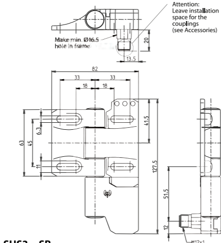
SHS3...SR...
