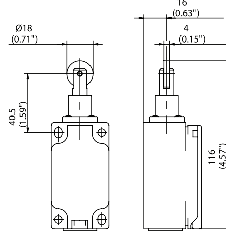
RIW (Form C)
