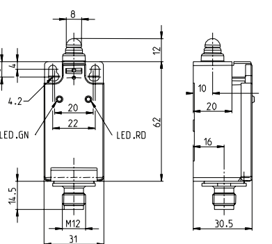
Drawing dimensions in mm
