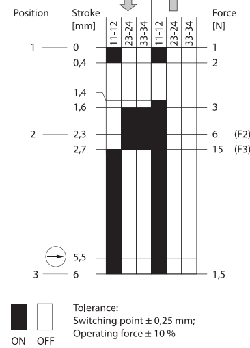
Switching diagram
