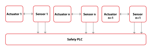
Series application
