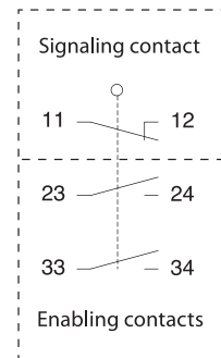
Circuit symbol
