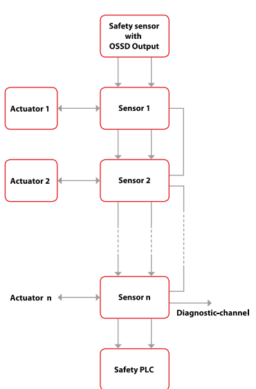
Series application
