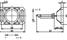
A4 ACTUATOR KEY 391.1702.231
