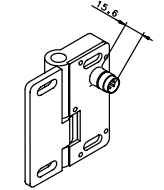
Connector M12 x 1
