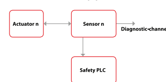
Individual application
