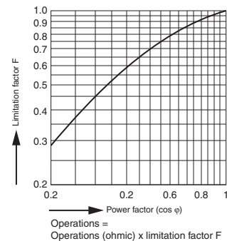
Limitation factor for inductive loads Operations = Operations (ohmic) x limitation factor F
