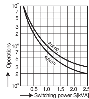
Mechanical life
