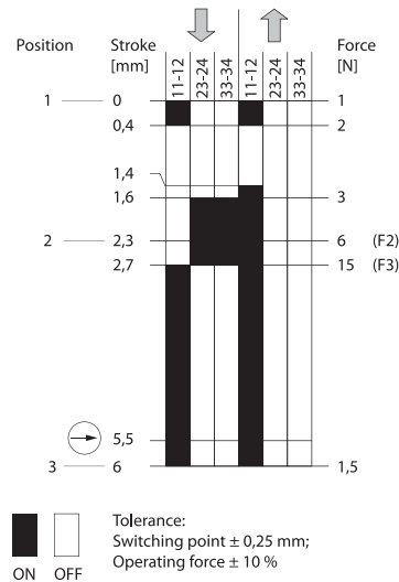
Switching diagram
