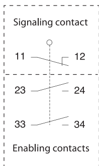
Circuit symbol
