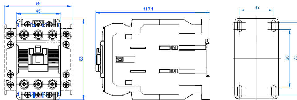
MC-32a~40a DC
