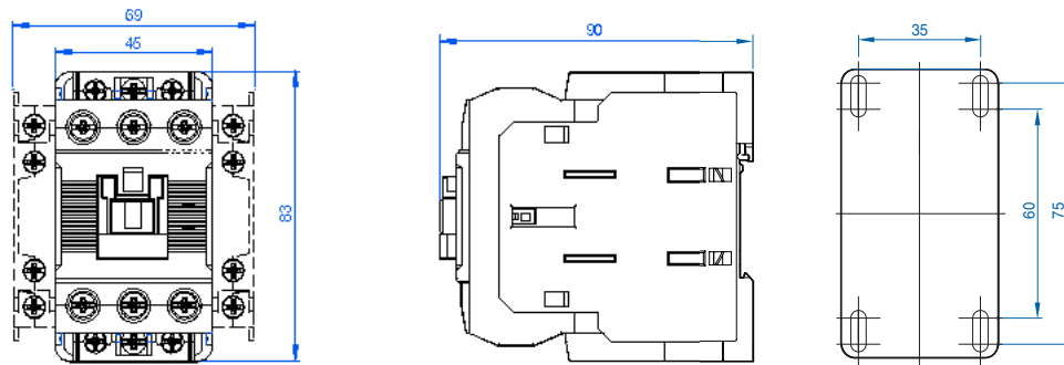
MC-32a~40a AC
