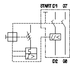
Connection Diagrams RUX
