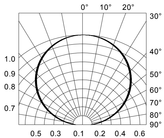
Fig.6-Radiation Diagram
