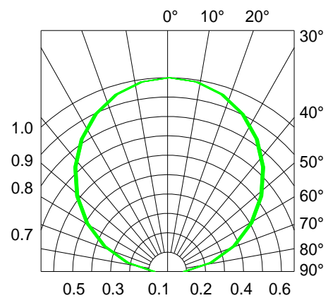
Fig.6-Radiation Diagram Ta=25°C
