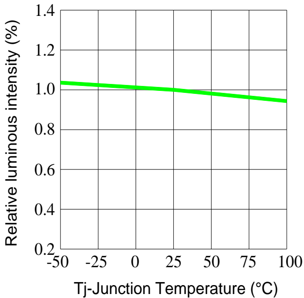
Fig.3-Relative Luminous Intensity vs.Junction Temperature
