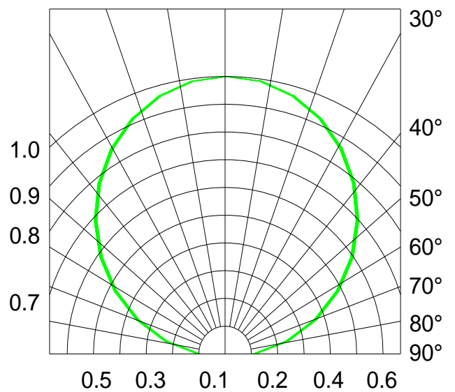
Fig.6-Radiation Diagram Ta=25°C
