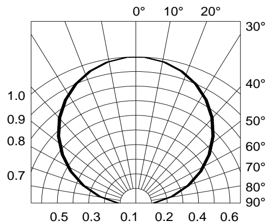
Fig.6-Radiation Diagram Ta=25°C
