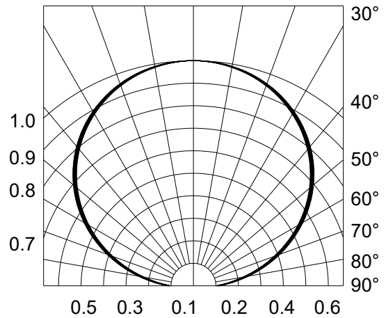
Fig.6-Radiation Diagram Ta=25°C
