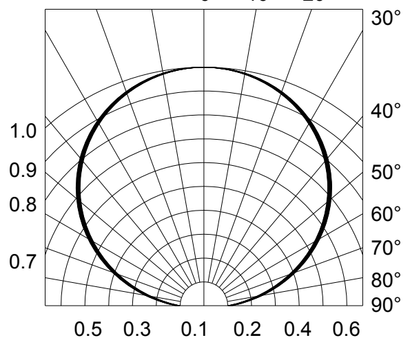
Fig.6-Radiation Diagram Ta=25°C
