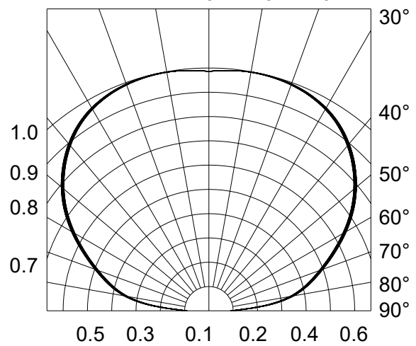
Fig.6-Radiation Diagram T_a=25^\circ\text{C}
