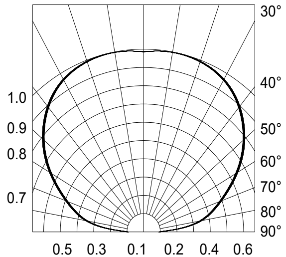
Fig.6-Radiation Diagram Ta=25°C
