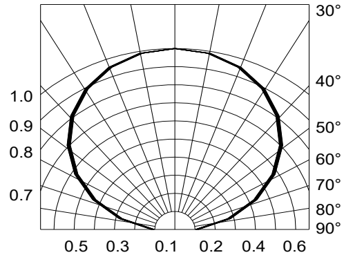
Fig.6-Radiation Diagram
