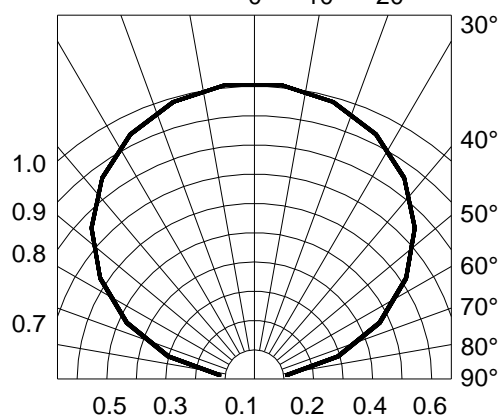
Fig.6-Radiation Diagram
