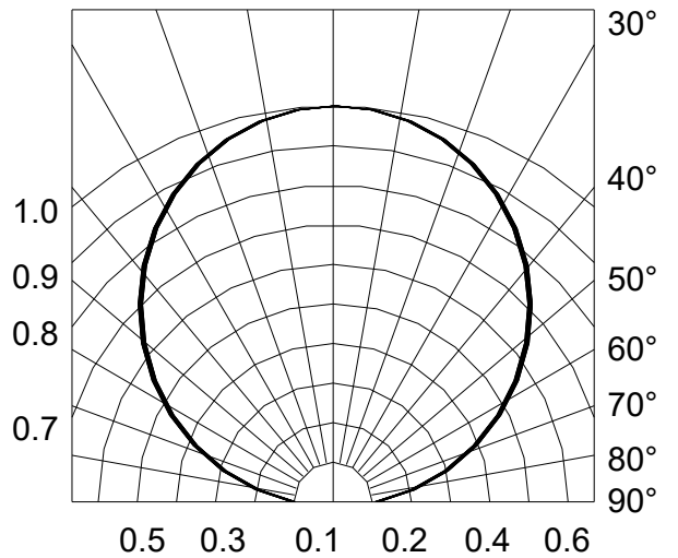
Fig.6-Radiation Diagram T_a=25^{\circ}\text{C}
