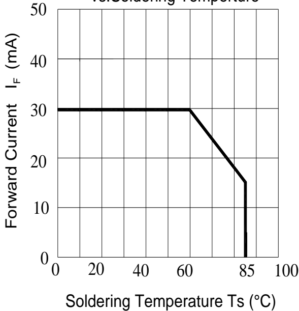
Fig.5-Max.Driving Forward Current vs.Soldering Temperature
