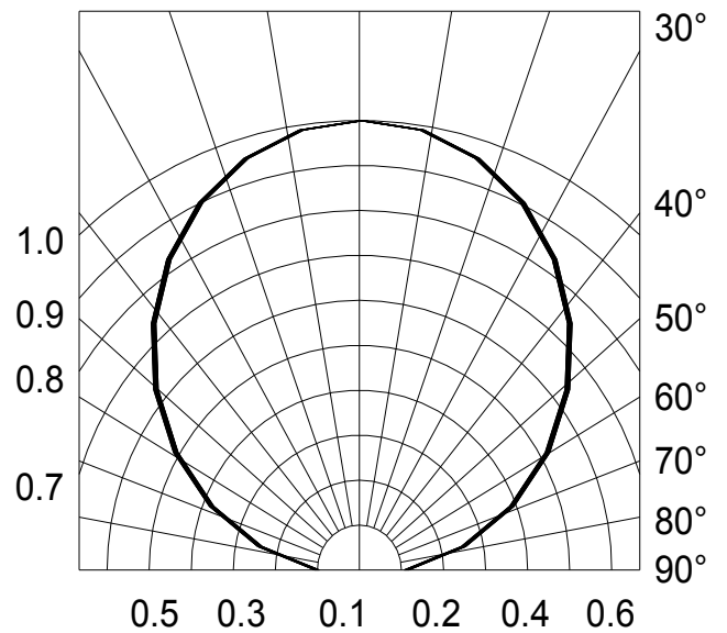
Fig.6-Radiation Diagram Ta=25°C
