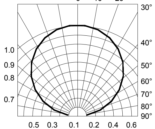
Fig.6-Radiation Diagram
