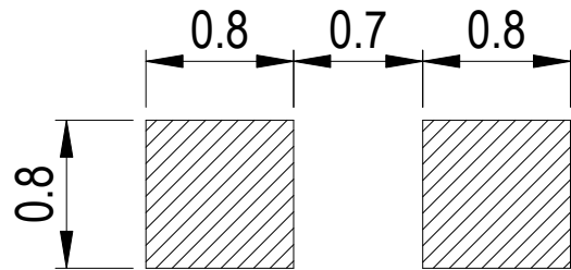
Recommended Solder Pad
