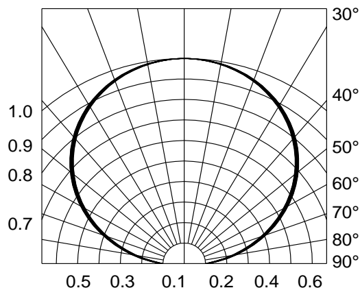
Fig.6-Radiation Diagram Ta=25°C
