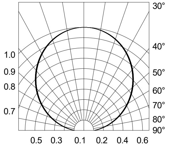
Fig.6-Radiation Diagram T_a=25^\circ\text{C}
