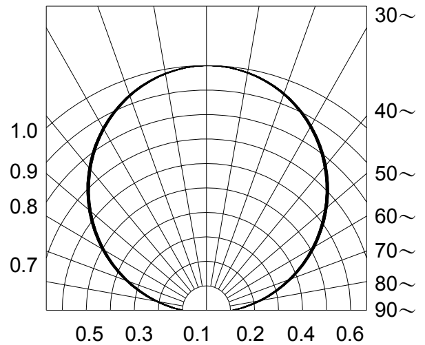
Fig.6-Radiation Diagram Ta=25-C 0~ 10~ 20~
