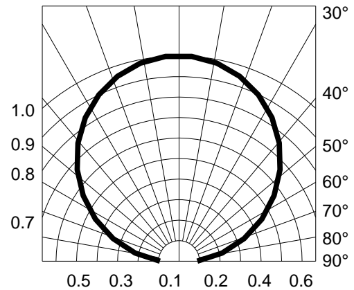
Fig.6-Radiation Diagram Ta=25°C
