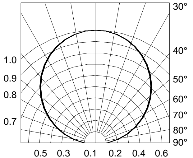
Fig.6-Radiation Diagram T_a=25^\circ\text{C}
