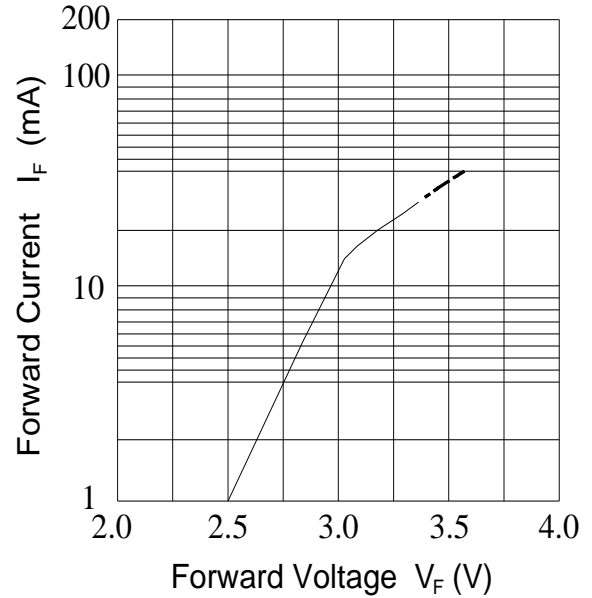
Fig.4-Forward Current vs. Forward Voltage T_a=25^\circ\text{C}
