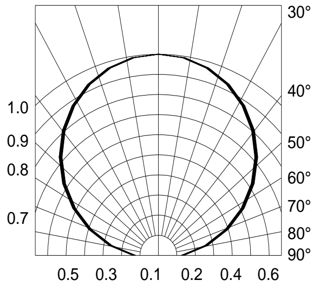
Fig.6-Radiation Diagram T_a=25^\circ\text{C}
