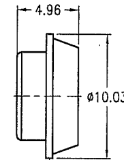
BRAID CLAMP
