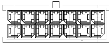
14 POS
