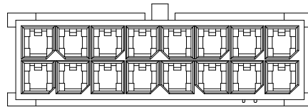
16 POS
