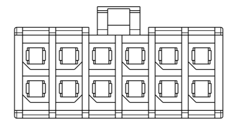
6POS6P(12P)
