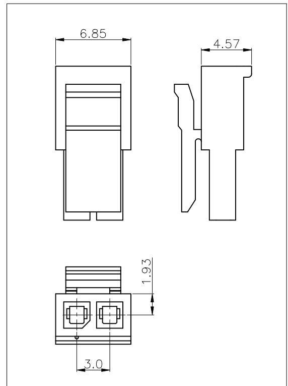
(2 CIRCUIT HOUSING)
