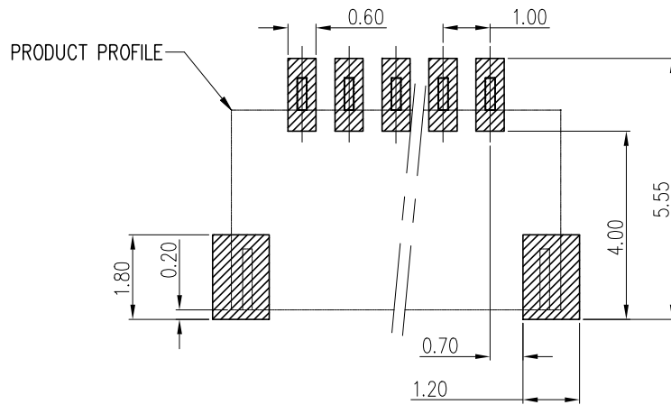
RECOMMENDED PCB LAYOUT GENERAL TOLERANCE \pm 0.05
