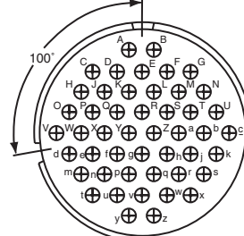
100° Rotation of 36-10
