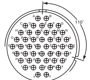
110° Rotation of 36-10
