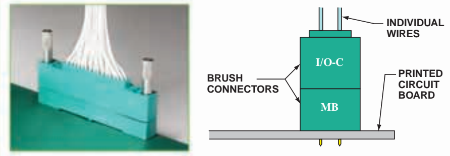
MB to I/O-C Discrete Wires to PCB
