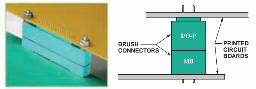
MB to I/O-P Mating Parallel Boards
