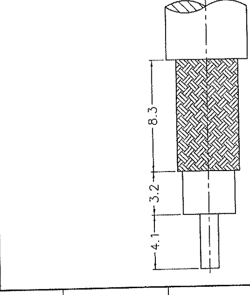
RECOMMENDED CABLE STRIPPING DIM'S (建議剝線尺寸)
