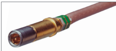
MIL-DTL-38999 LJT-R, JT-R, TV-R, SJT-R MS Type, Coax Size 12 Socket Assembled Contact
