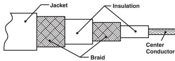
Cable Illustration - Triax Contact
