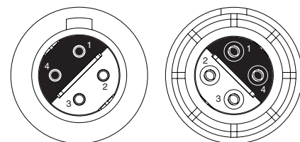
PIN CONTACT MATING FACE SOCKET CONTACT MATING FACE Differential Pairs: 1 & 4, 2 & 3
