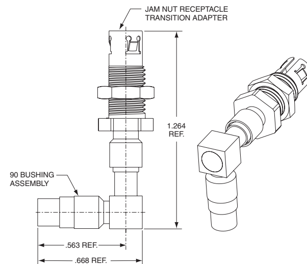
90° BUSHING ASSEMBLY WITH WIRED MICRO DIFFERENTIAL JAM NUT RECEPTACLE TRANSITION ADAPTER
