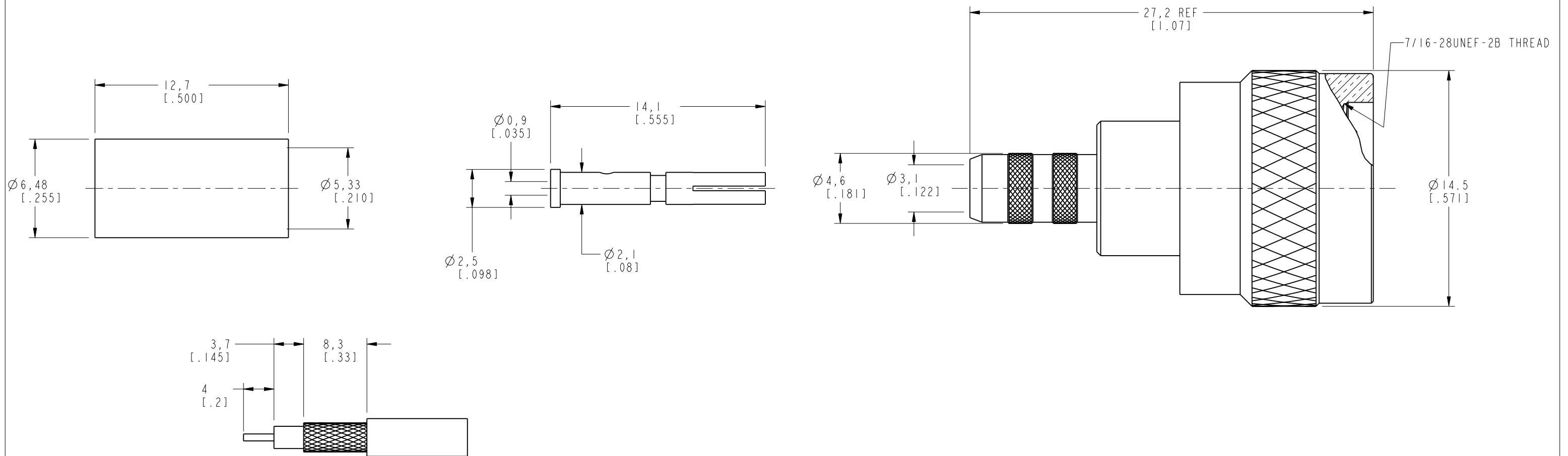
RECOMMENDED CABLE STRIPPING DIMENSIONS SCALE 2.000
