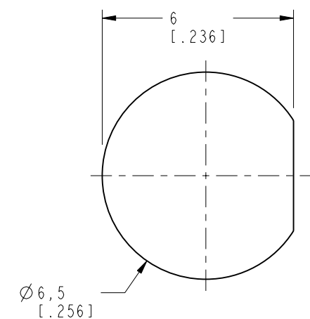
RECOMMENDED MOUNTING HOLE DIMENSIONS
