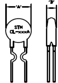
KINKED LEADS
