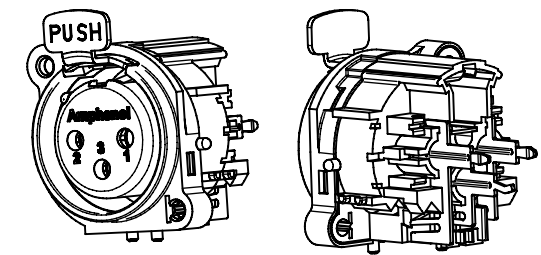
3D VIEW (1:1)
