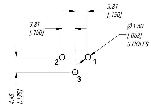
PCB LAYOUT LAYOUT TOLERANCE : ±0.05 [±.002 in]
