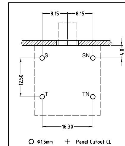
PCB LAYOUT
