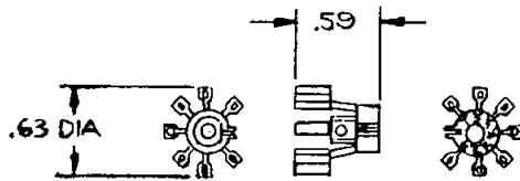
A AP-107-3B CABLE HOLDER PLUG
