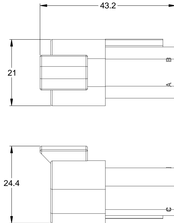
REFERENCE DIMENSIONS - ASSEMBLED
